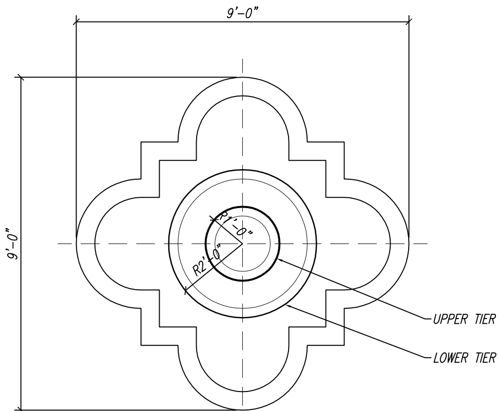
PLAN VIEW
