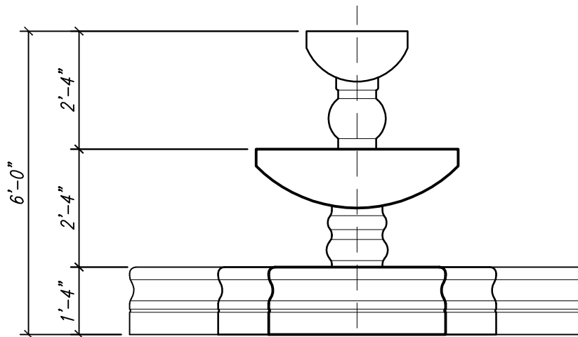
ELEVATION VIEW
