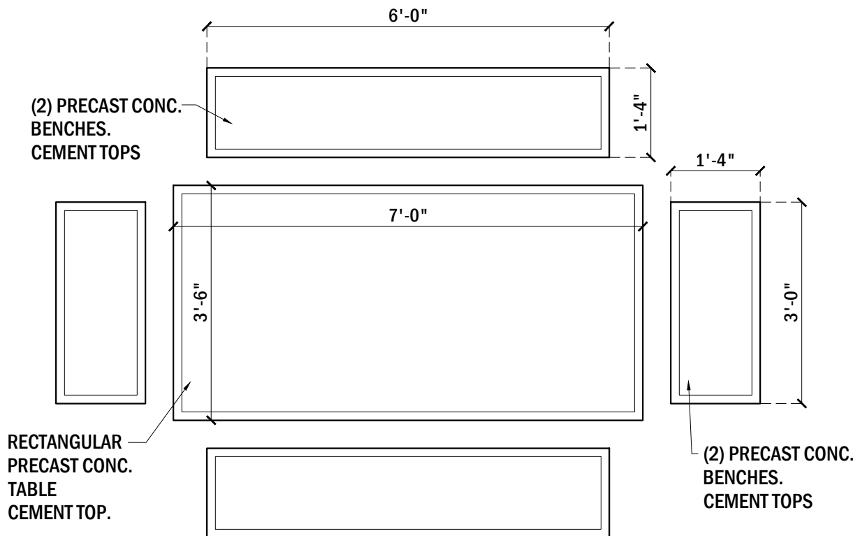
PLAN VIEW, TABLE #616
