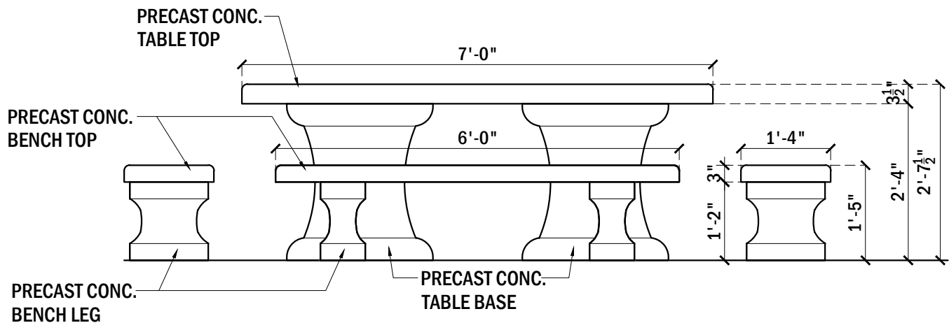
ELEVATION VIEW, TABLE #616
