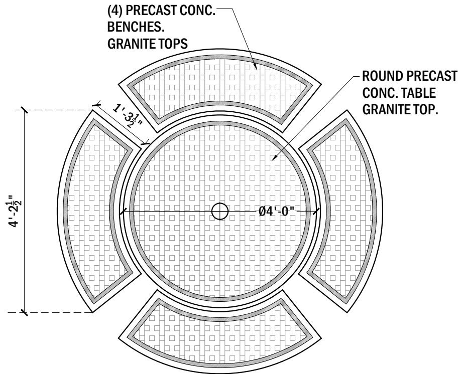
PLAN VIEW, TABLE #612
