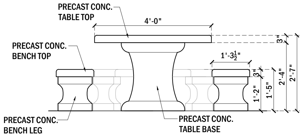
ELEVATION VIEW, TABLE #612
