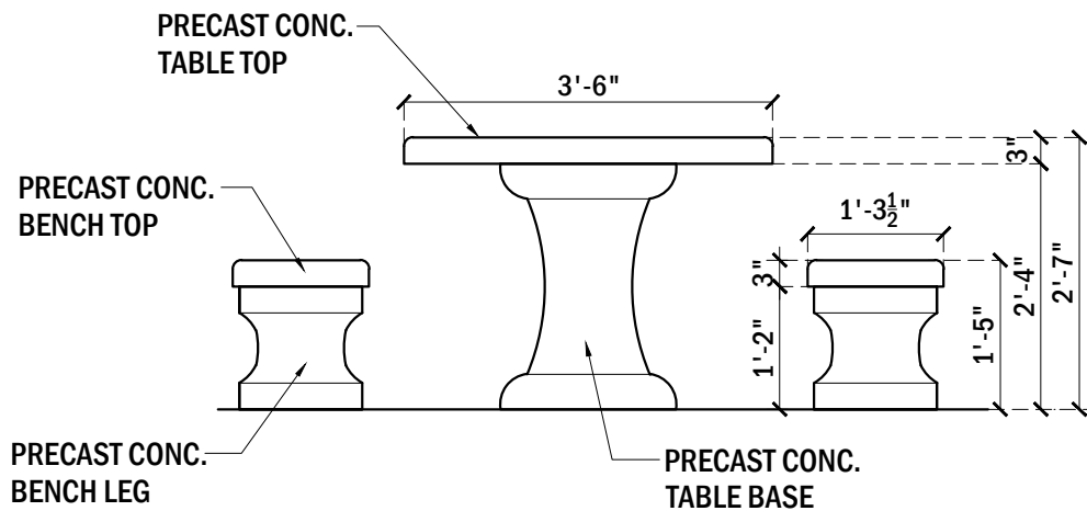
ELEVATION VIEW, TABLE #605
