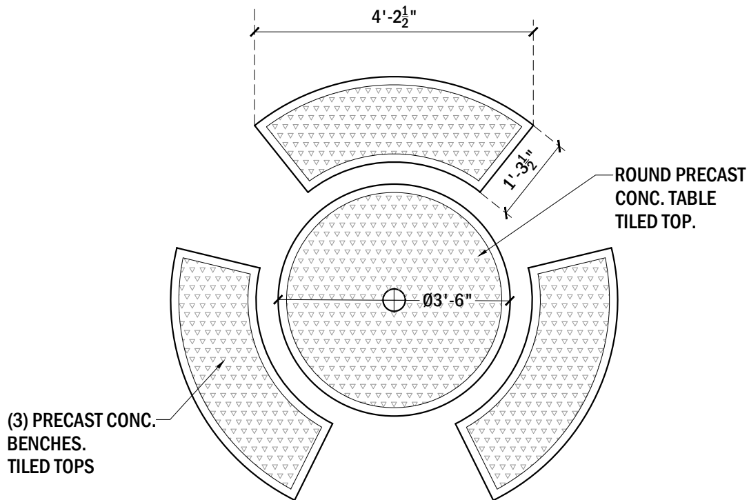
PLAN VIEW, TABLE #605
