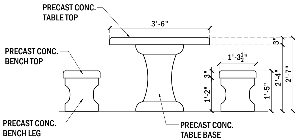
ELEVATION VIEW, TABLE #604
