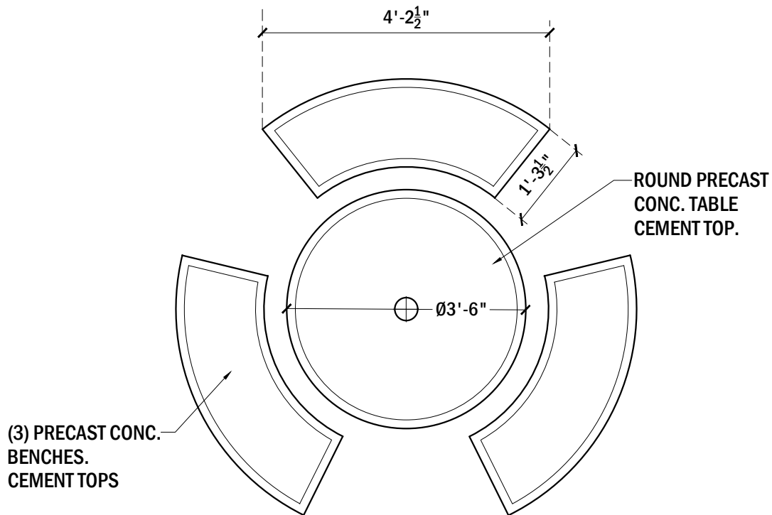
PLAN VIEW, TABLE #604
