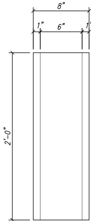
PLAN VIEW
