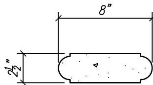
PROFILE VIEW
