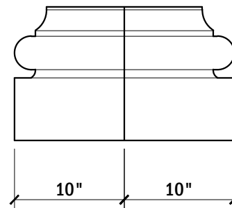
PROFILE VIEW
