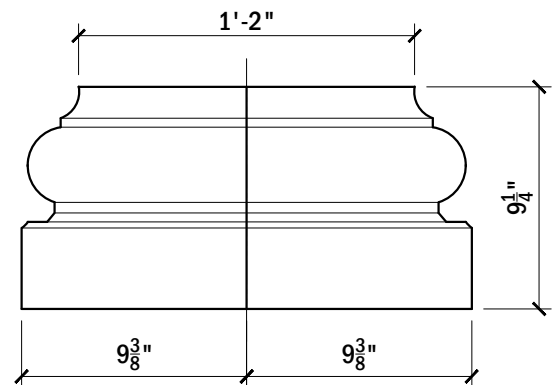
PROFILE VIEW
