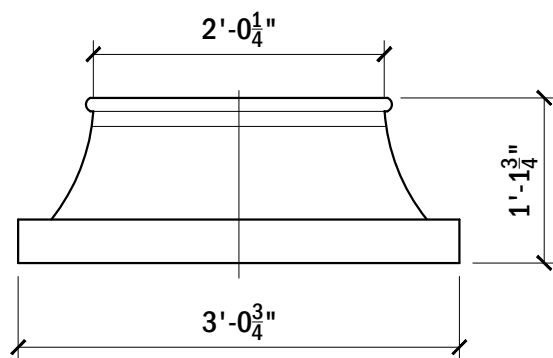
ELEVATION VIEW
