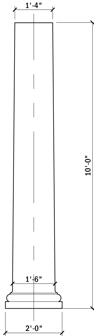
ELEVATION VIEW
