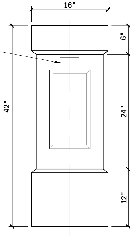
ELEVATION VIEW
