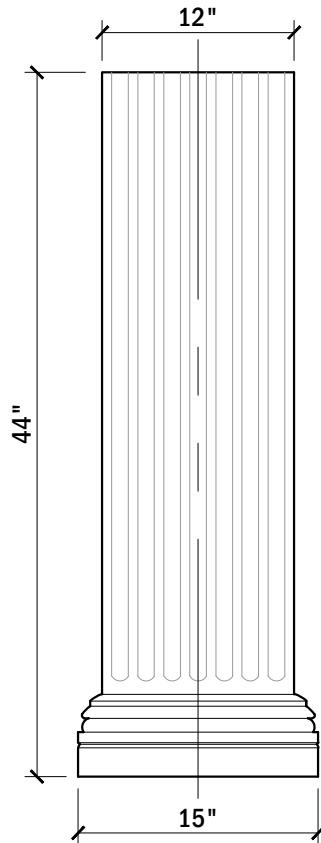
ELEVATION VIEW
