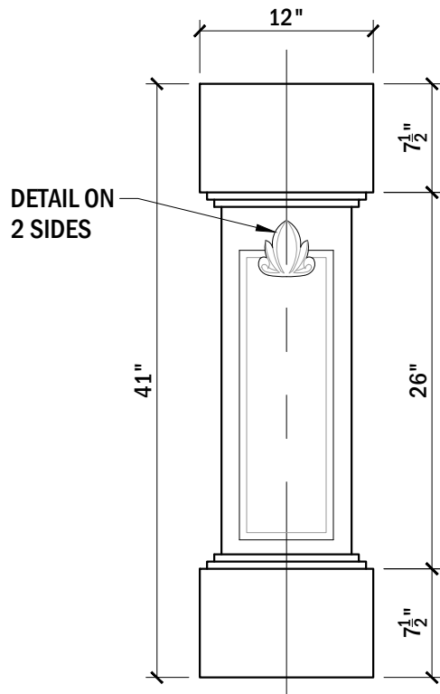
ELEVATION VIEW
