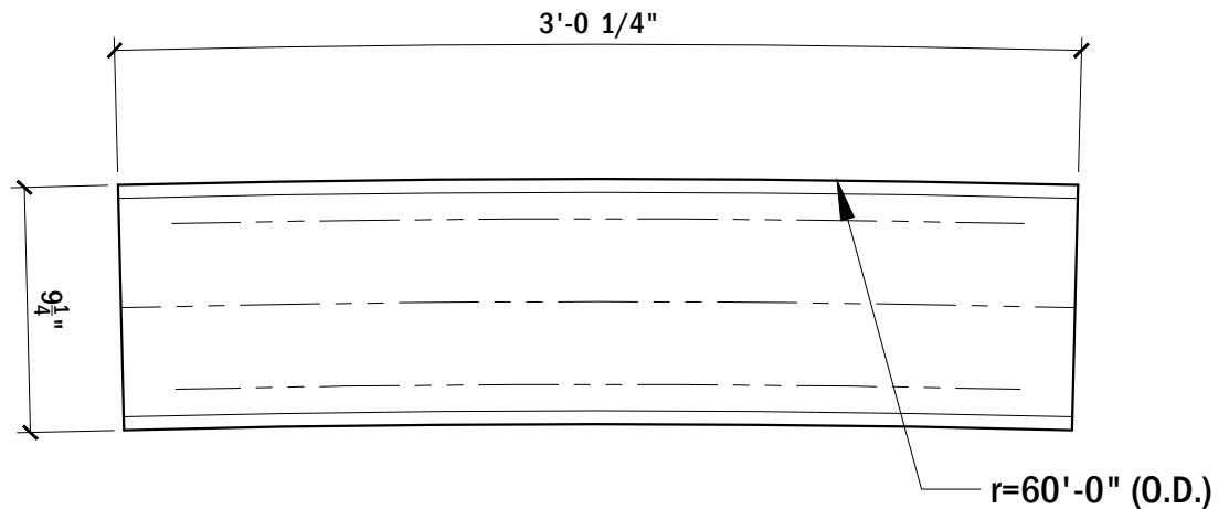
PLAN VIEW, BASE RAIL #159
