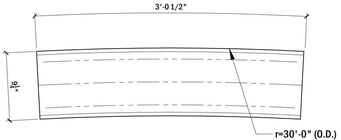
PLAN VIEW, TOP RAIL #157
