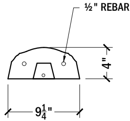
SIDE VIEW, TOP RAIL # 147
