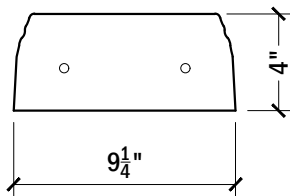
SIDE VIEW BASE RAIL #140
