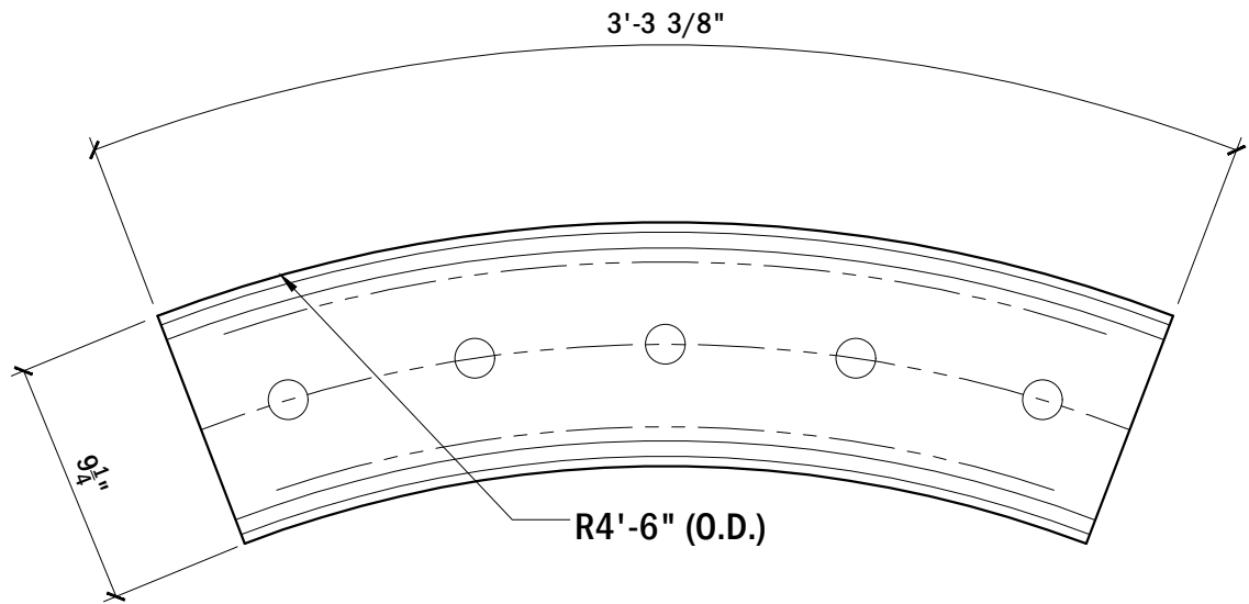
TOP VIEW, BASE RAIL #140
