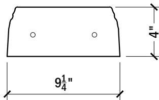
SIDE VIEW BASE RAIL #139
