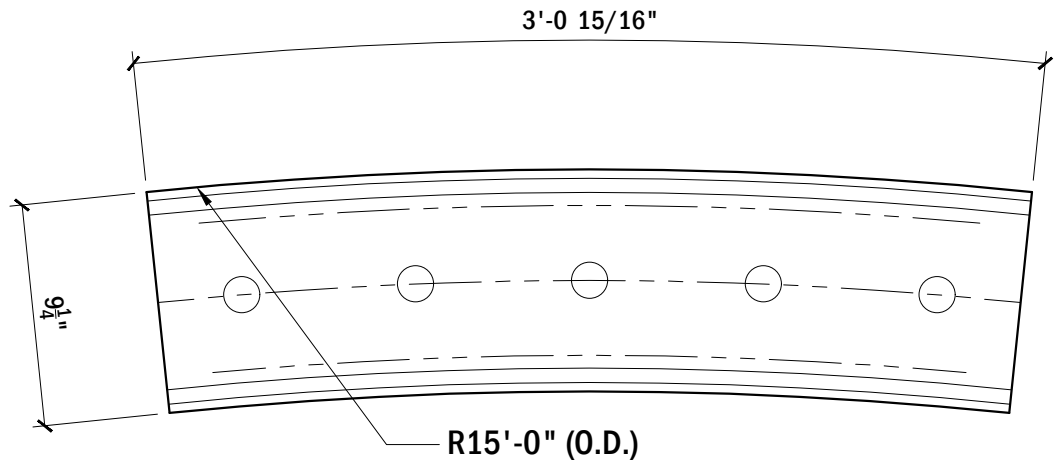
TOP VIEW, BASE RAIL #139
