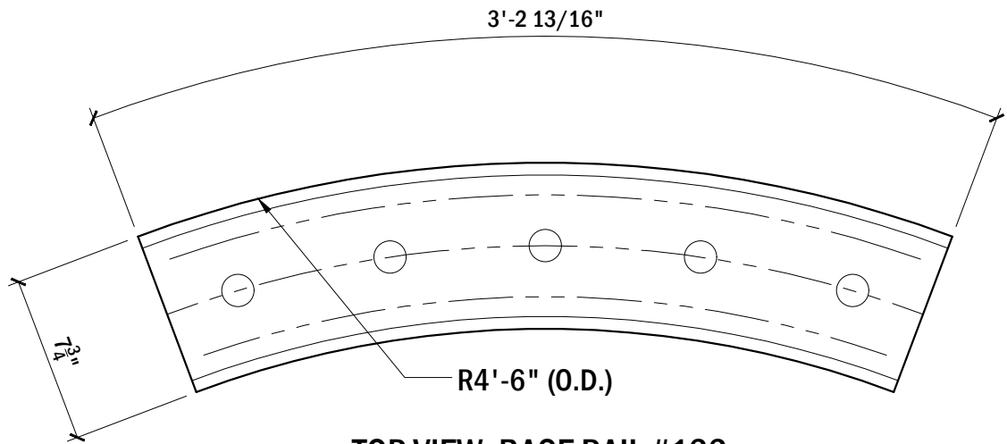
TOP VIEW, BASE RAIL #133
