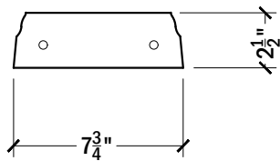
SIDE VIEW BASE RAIL #133
