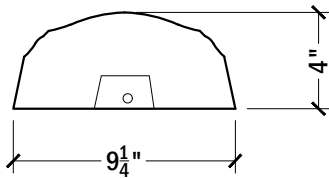
SIDE VIEW TOP RAIL #131
