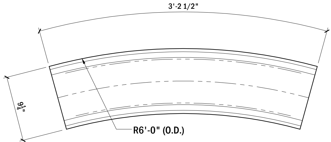
TOP VIEW, TOP RAIL #131
