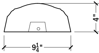
SIDE VIEW TOP RAIL #130
