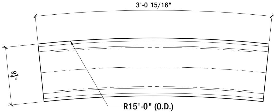
TOP VIEW, TOP RAIL #130
