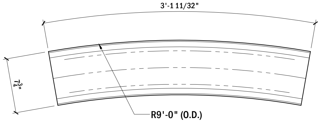
TOP VIEW, TOP RAIL #126
