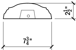
SIDE VIEW TOP RAIL #126
