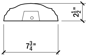
SIDE VIEW TOP RAIL #124
