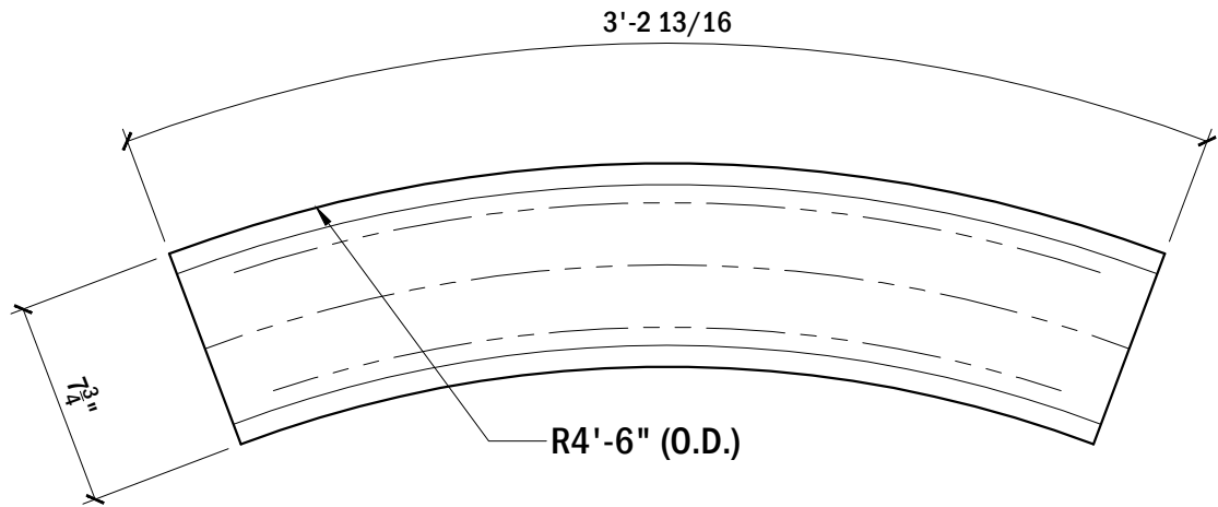
TOP VIEW, TOP RAIL #124
