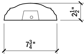
SIDE VIEW TOP RAIL #123
