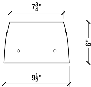
SIDE VIEW BASE RAIL #121
