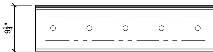
TOP VIEW, BASE RAIL #137
