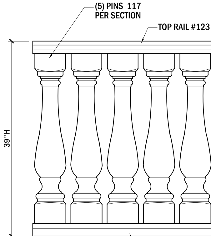
ELEVATION VIEW
