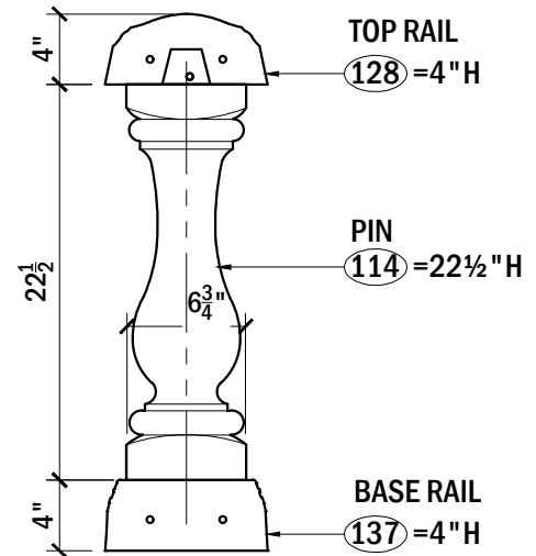
PROFILE VIEW
