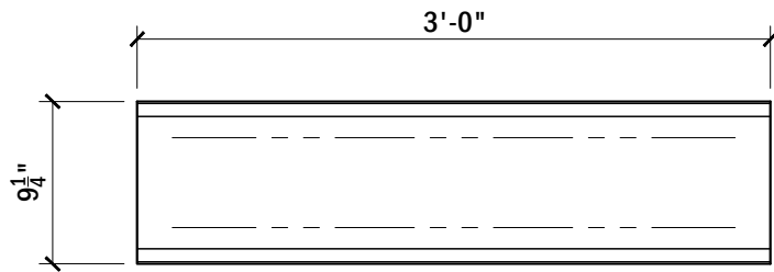
TOP VIEW, TOP RAIL # 128
